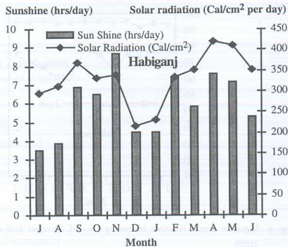
Fig. 3. Monthly solar radiation (Cal/cm 2 /day) and sunshine (hrs/day) of Gazipur and other three regional stations of BTRI, from July 2008 to June 2009.
